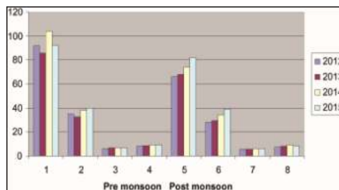
Fig - 3: Diagrammatic representation of TSPM, PM 10 , SO 2 and NO x levels of Puthu kudieruppu sampling station during 2012-2015
