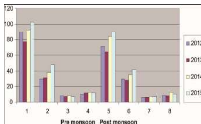
Fig – 2: Diagrammatic representation of TSPM, PM 10 , SO 2 and NO x levels of Mantharakippam sampling station during 2012 - 2015
